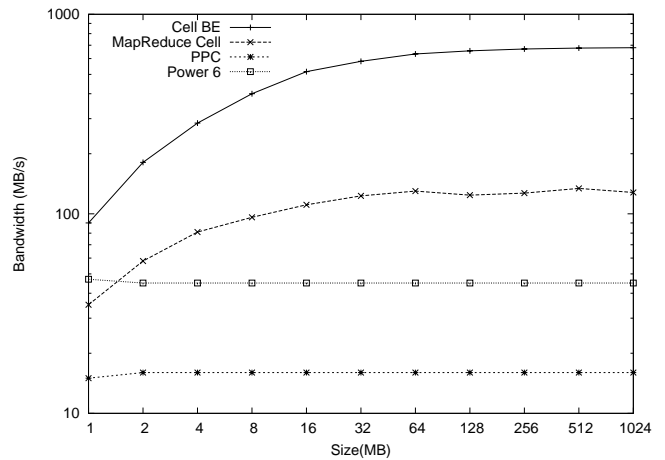
Fig. 2. Raw node encryption performance
