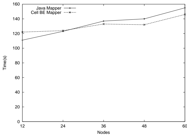
Fig. 4. Distributed encryption performance: proportional data set
