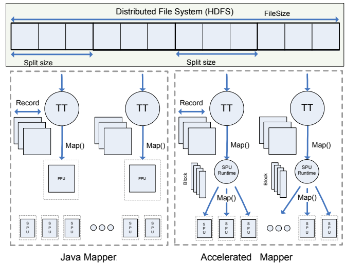
Fig. 3. Data distribution model
