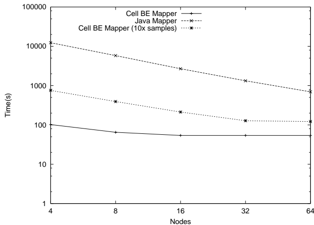
Fig. 8. Distributed Pi estimation performance: 10e+11 samples
