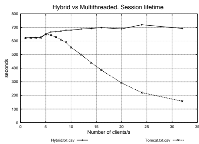
Figure 8: Lifetime comparison for the sessions completed successfully under a dynamic content workload
