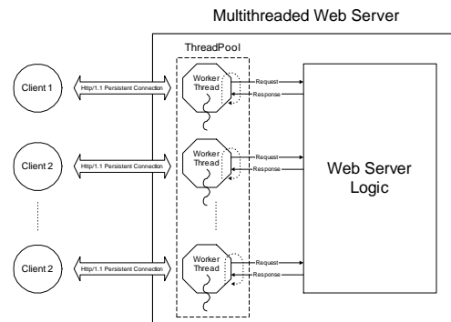
Figure 1: Multithread architecture diagram
