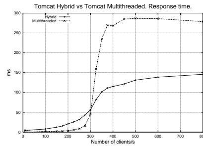
Figure 4: Response time under an static content workload
