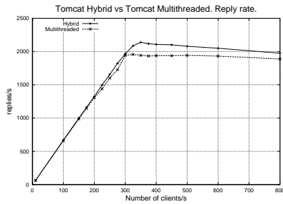
Figure 3: Throughput comparison under an static content workload
