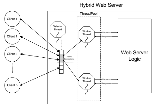
Figure 2: Hybrid architecture diagram
