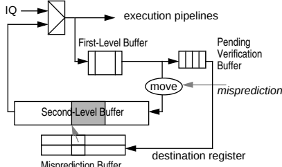
Figure 9: Recovery-Buffer organization.
