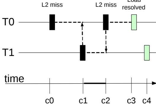
Fig. 10. Timing when a thread with high L2 miss rate is executed
