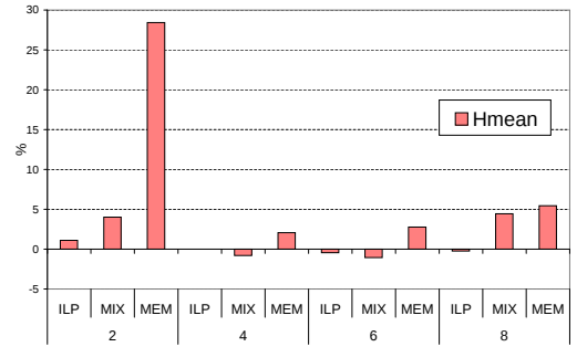
(b) Hmean results
