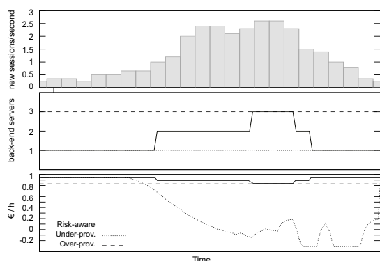
Fig. 2. CSP profit with a one-day typical workload.
