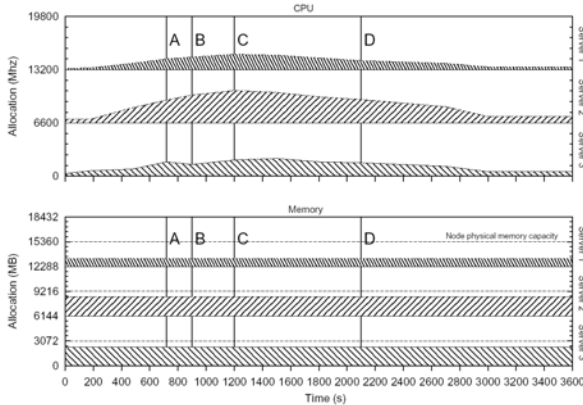
Figure 1. Per-node CPU and memory consumption without memory compression
