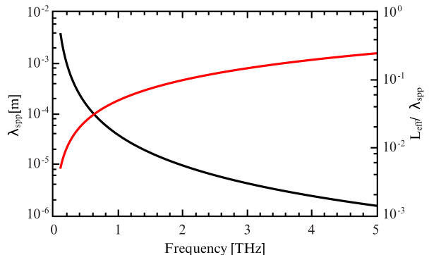
Figure 5: Logarithmic plot of the plasmon wavelength (black line, left vertical axis) and the ratio of the propagation length to the plasmon wavelength (red line, right vertical axis) in a free-standing graphene layer as a function of frequency. The frequency ranges from 0.1 to 5 THz.
