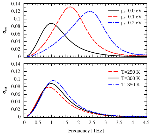
Figure 8: Dependence of the antenna resonant frequency on the electrostatic bias at T = 300 K (top) and on the temperature at \mu_c = 0 eV (bottom). L = 1 \mu\text{m} , W = 0.5 \mu\text{m} , D = \infty and \epsilon=11.9 .
