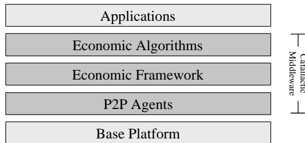
Figure 3. A layered architecture for resource allocation
