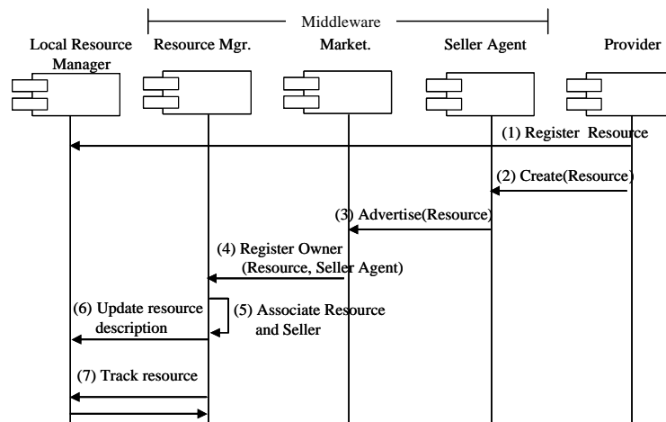
Figure 4. Registering Agents and resources.
