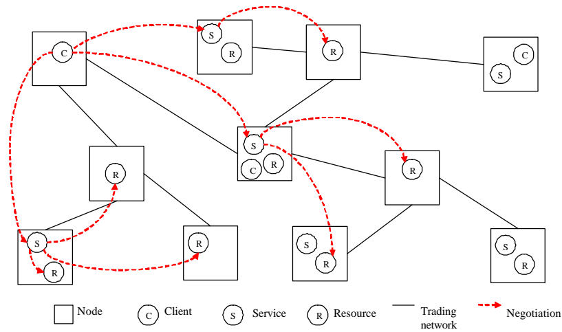
Figure 2. Decentralized allocation of resources in an ALN.
