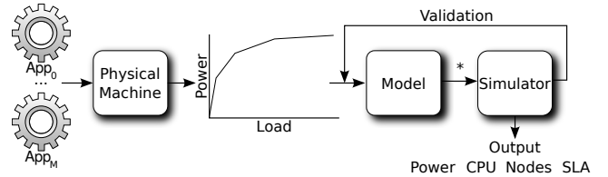
Figure 2: Simulator workflow
