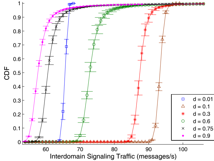
Fig. 7. fP2P-HN Inter-Domain signalling traffic
