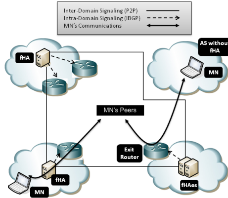
Fig. 1. Overview of the fP2P-HN architecture
