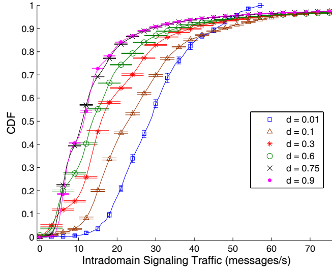
Fig. 8. fP2P-HN Intra-domain signalling traffic
