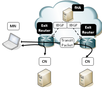
Fig. 3. Data Packet Forwarding
