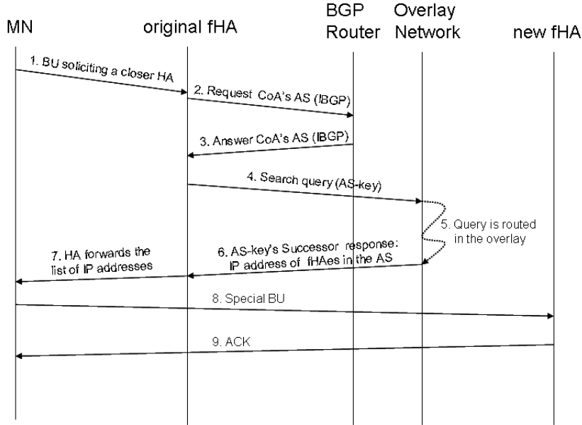
Fig. 2. fHA Discovery Phase in the fp2P-HN architecture
