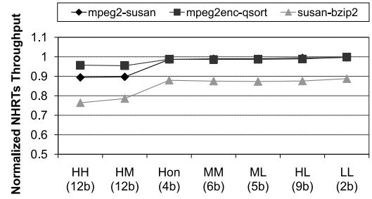
Figure 12: Normalized Throughput of NHRTs. The numbers in parenthesis are the number of L2 banks required by the HRTs
