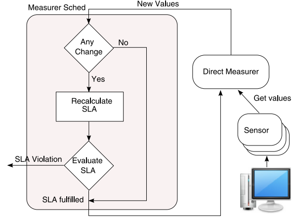
Fig. 2. SLA evaluation cycle.
