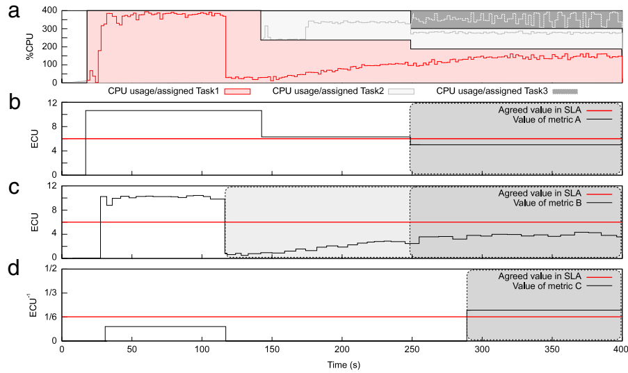
Fig. 3. Comparison of CPU-based SLA metrics. (a) CPU assignment and usage for Task 1, 2, and 3. (b) Fulfillment of SLA metric A for Task 1. (c) Fulfillment of SLA metric B for Task 1. (d) Fulfillment of SLA metric C for Task 1.
