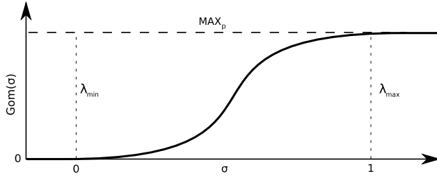
Fig. 1. Gompertz function for SLA penalties.
