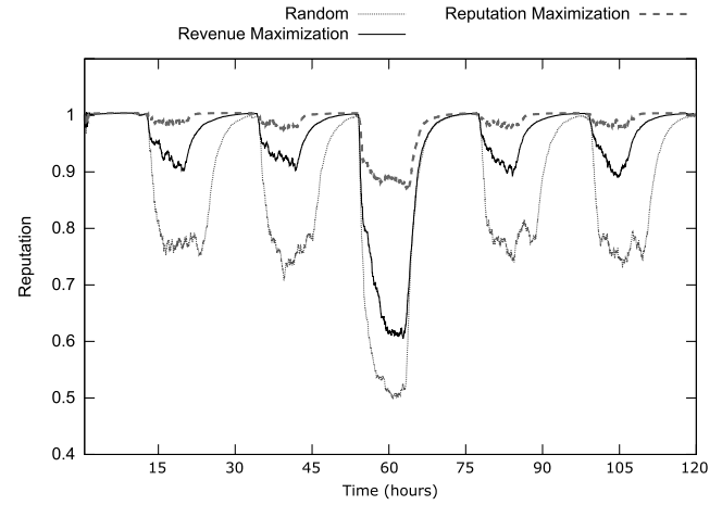
Fig. 5. Evolution of reputation for three types of providers.
