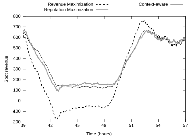
Fig. 8. Spot revenue for three types of providers, including context-aware policy switching, during and after an outage.
