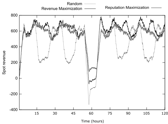
Fig. 6. Spot revenue of three types of providers.
