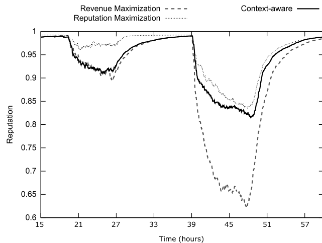
Fig. 7. Evolution of reputation for three types of providers, including context-aware policy switching.
