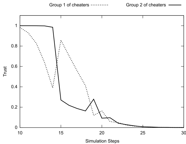
Fig. 12. Evolution of trust for peers that perform an oscillation attack.
