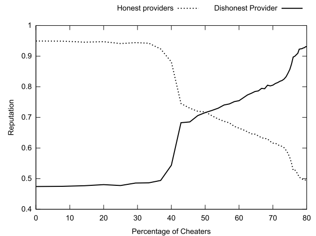
Fig. 13. Reputation of providers under a basic orchestrated attack.
