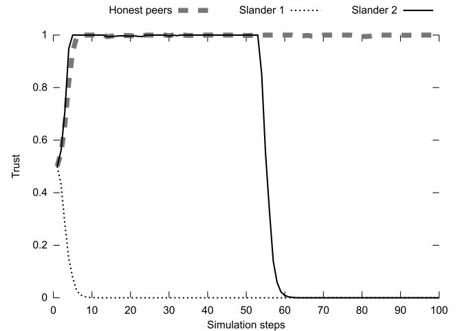
Fig. 10. Evaluation of trust to peers that perform Slandering.
