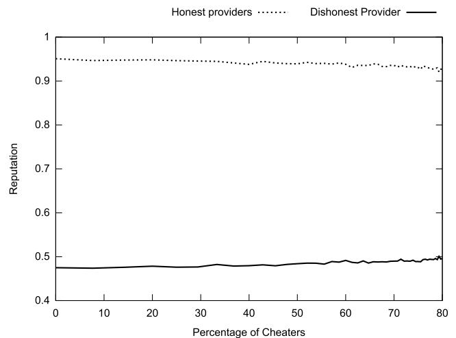
Fig. 11. Reputation of providers under oscillation attacks.
