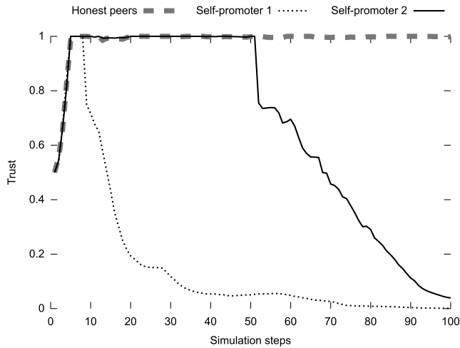
Fig. 9. Evaluation of trust to peers that perform Self-promoting.
