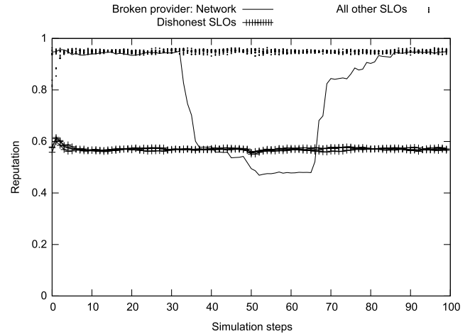
Fig. 4. Reputation of providers upon failures and dishonest behaviours.
