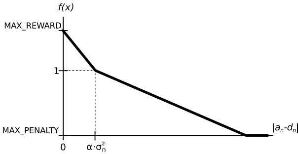
Fig. 2. Function to multiply the trust to a given peer, based on its previous report.
