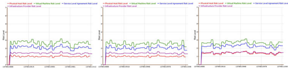
Fig. 10. Three Concurrent heterogeneous services, five VMs.
