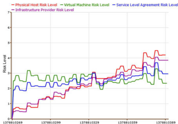
Fig. 7. 1-10 Homogeneous concurrent services, service profile two, five VM per service.
