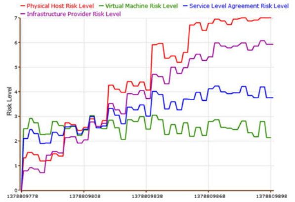
Fig. 8. 1-10 Homogeneous concurrent services, service profile three, five VM per service.
