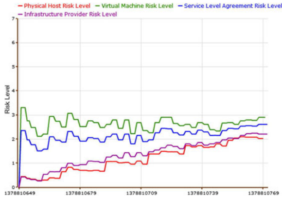
Fig. 6. 1-10 Homogeneous concurrent services, service profile one, five VM per service.
