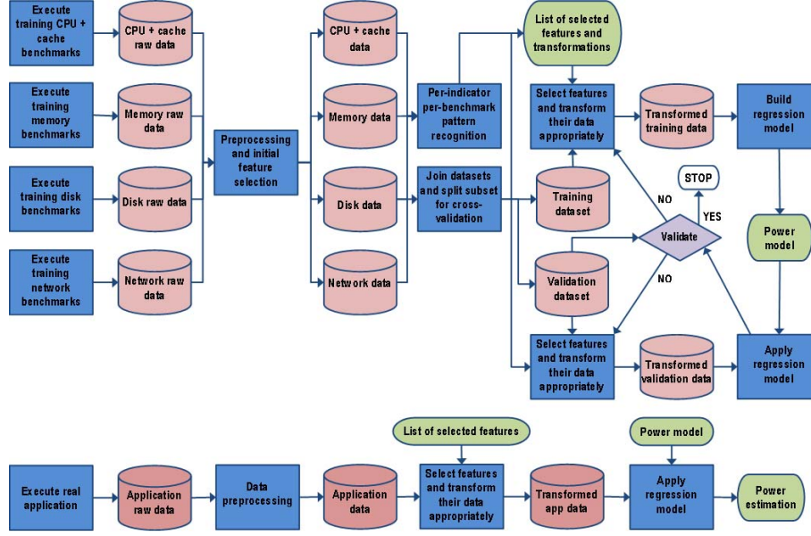
Figure 2: Model generation (top) and validation (bottom) procedures
