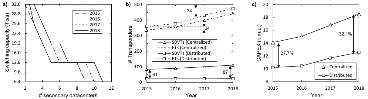
Fig. 3. Average switching capacity (a), total number of FTs and SBVTs installed (b) and total network CAPEX (c).
