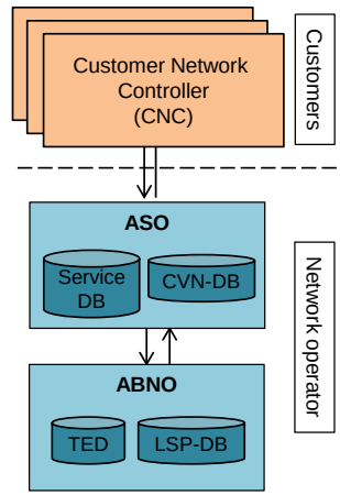
Fig. 2. Management architecture
