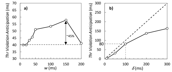
Fig. 5: Threshold violation anticipation vs. w (a) and \delta (b)
