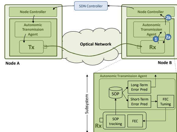
Fig. 1: Autonomic transmission and detail of receiver side
