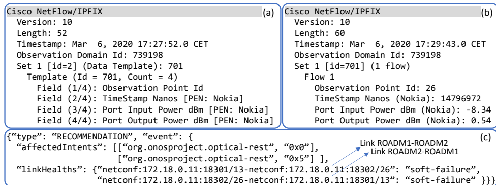
Figure 4. Relevant messages exchanged: (a) IPFIX template record, (b) IPFIX data record (message 1), and (c) JSON recommendation from MDA to ONOS (message 3).
