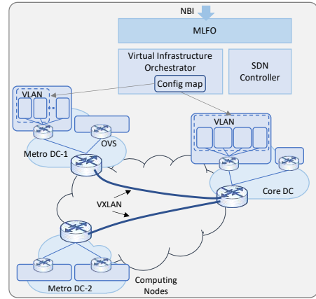
Fig. 3: Architecture of the solution.
