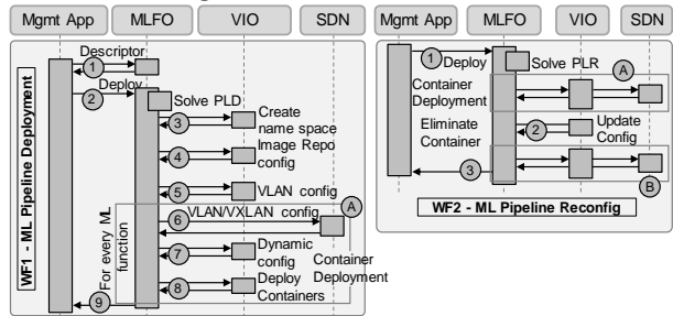
Fig. 4: Deployment and reconfiguration.
