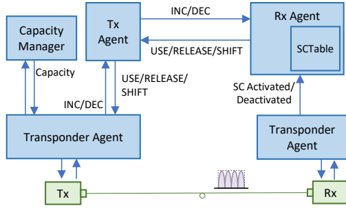
Figure 2: Relation between MAS and transponder agents
