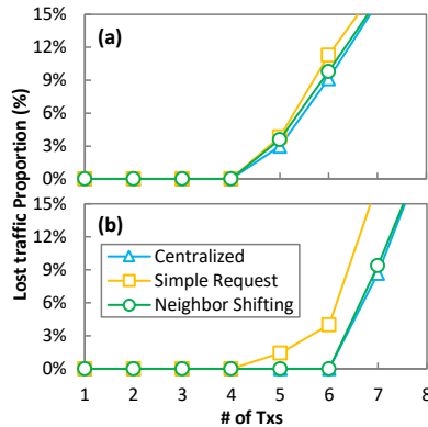
Figure 4: MAS vs Centralized
