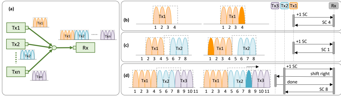
Figure 1: MP2P connectivity based on DSCM (a). SC allocation upon Tx1 request (b) and (c). Neighbor shifting (d).
