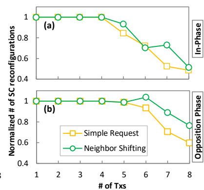
Figure 5: SC reconfigurations
