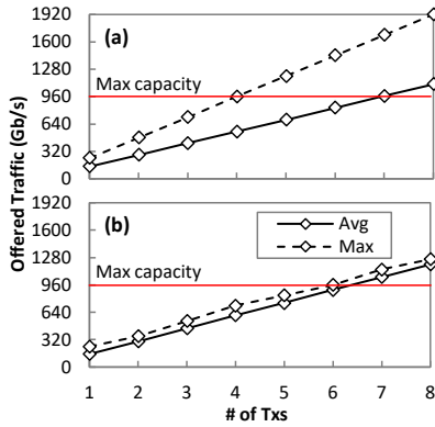
Figure 3: Offered Traffic at Rx
