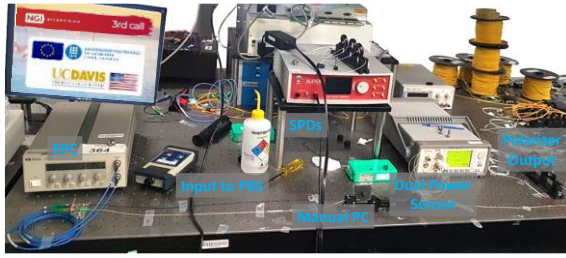
Figure 3. Experimental Testbed.
