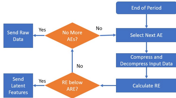
Figure 3. ACC procedure.
