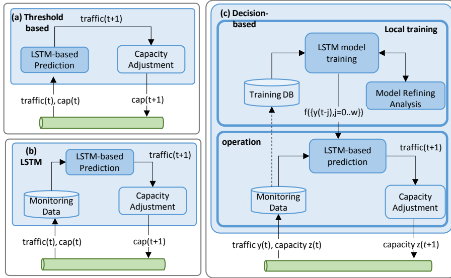
Figure 1: (a) Threshold-based, (b) LSTM, and (c) Decision-based.
