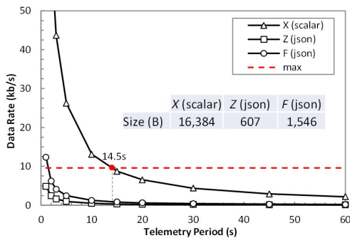
Figure 5. Telemetry data rate vs period.
