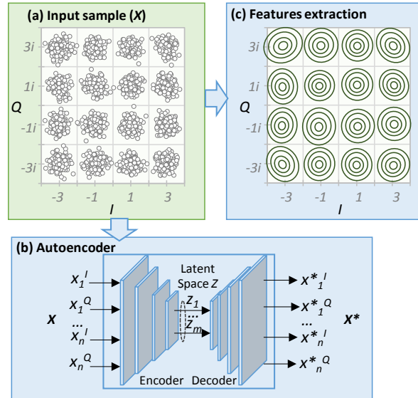
Figure 3: (a) Constellation sample; (b) Use of autoencoders; (c) Supervised features extraction.
