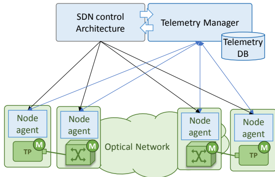
Figure 1. Overall network architecture.
