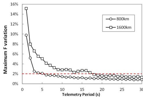
Figure 6. Aggregation error vs telemetry period.
