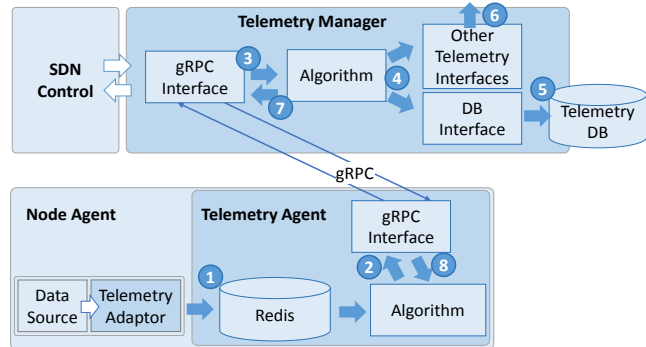
Figure 2. Proposed telemetry architecture.
