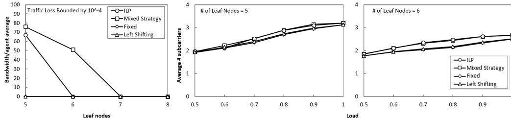
Fig. 3: a) Average bandwidth supported by a leaf node with loss below 10^{-4} . Average number of occupied SCs per leaf for (b) 5 leaf nodes, (c) 6 leaf nodes.
