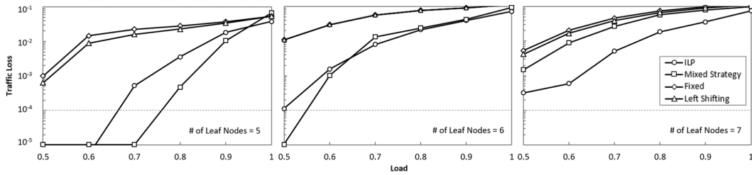
Fig. 2: Percent traffic loss for (a) 5 leaf nodes, (b) 6 leaf nodes, and (c) 7 leaf nodes.
