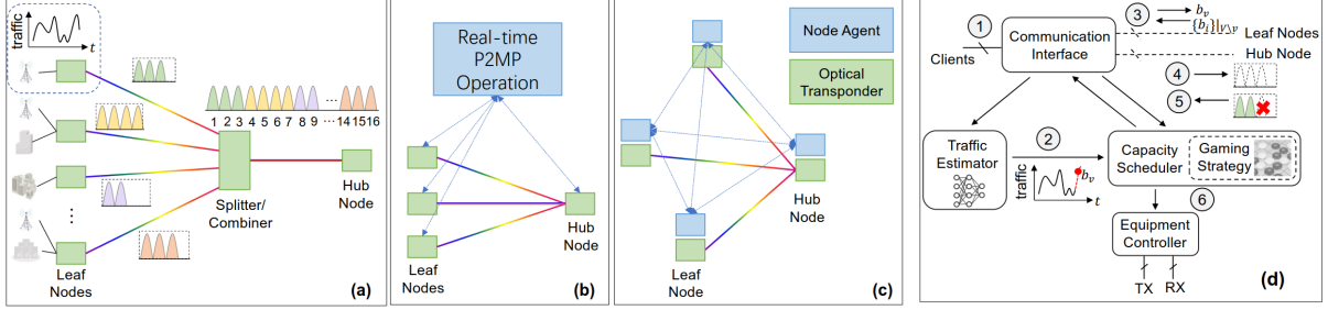
Fig. 1: (a) Illustration of P2MP communication based on DSCM, (b) real-time P2MP operation, (c) node intelligent agents centralized operation, and (d) operation principle of a leaf agent.
