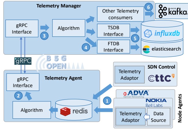
Fig. 2: B5G-OPEN Telemetry architecture and workflow
